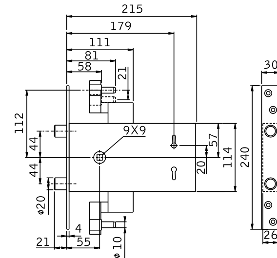
ASSA 5970 Measurement in mm
