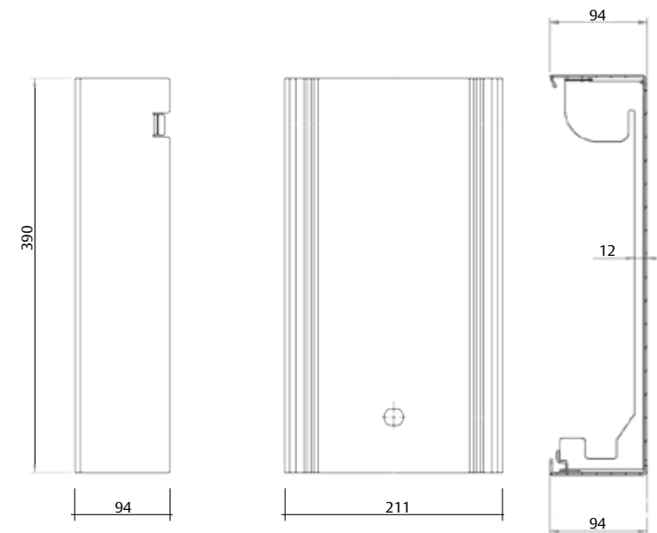
Dimension drawing LCU6516II
