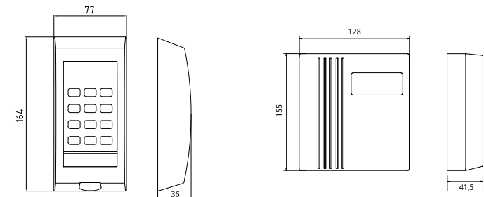
Dimension drawing
