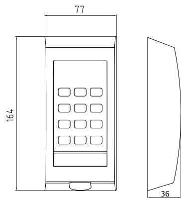
Dimension drawing
