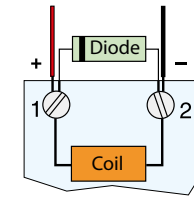
A protective diode should be connected; the stripe on the diode should be wired to + (all)
