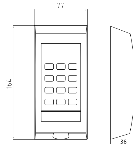
Dimension drawing
