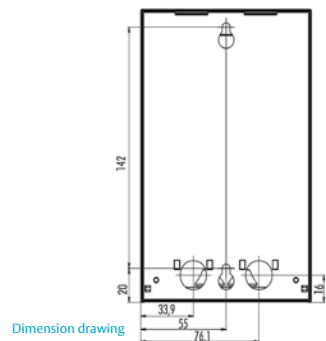
Dimension drawing
