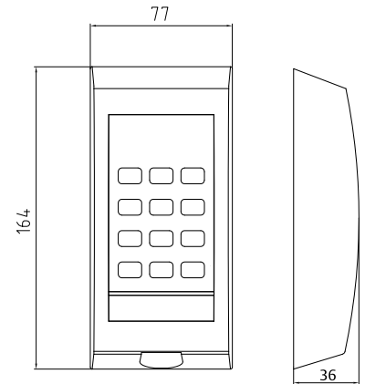
Measurement in mm, not proportional
