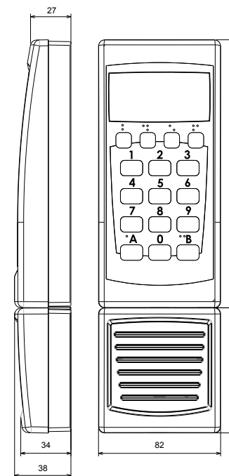
Dimension drawing
