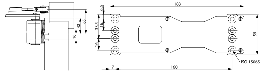
Mounting plate A120
