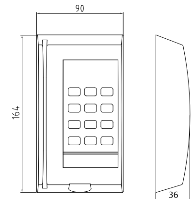
Dimension drawing
