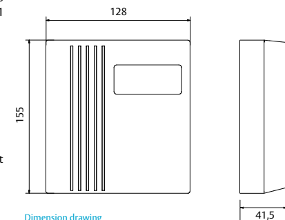
Dimension drawing
