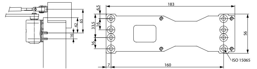
Mounting plate A120
