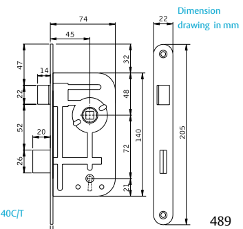
Dimension drawing in mm
