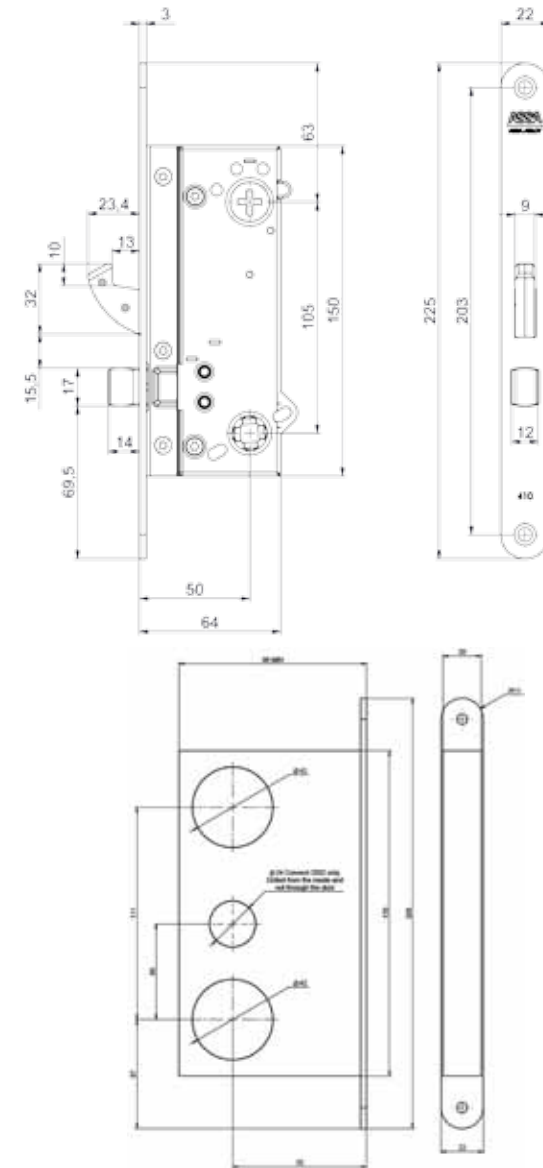
Dimension drawing, Connect 410-70, 410-70 MA
