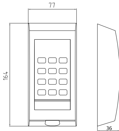
Dimension drawing
