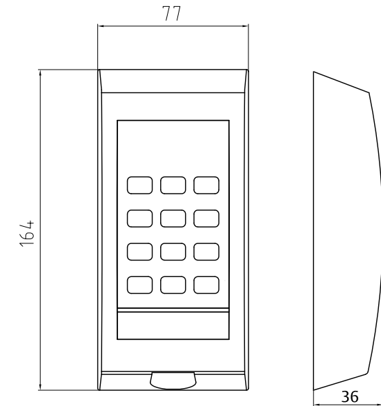
Dimension drawing
