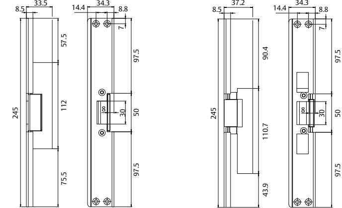
Faceplate 545 Faceplate 745
