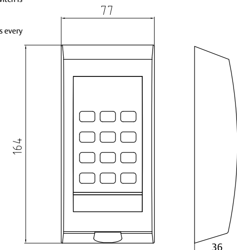
Measurement in mm, not proportional
