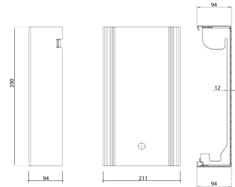
Dimension drawing LCU9017II
