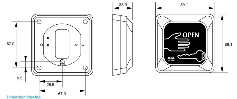
Dimension drawing
