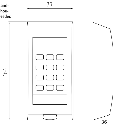
Dimension drawing
