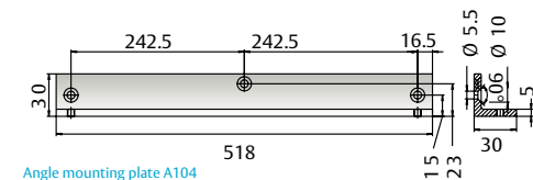
Angle mounting plate A104
