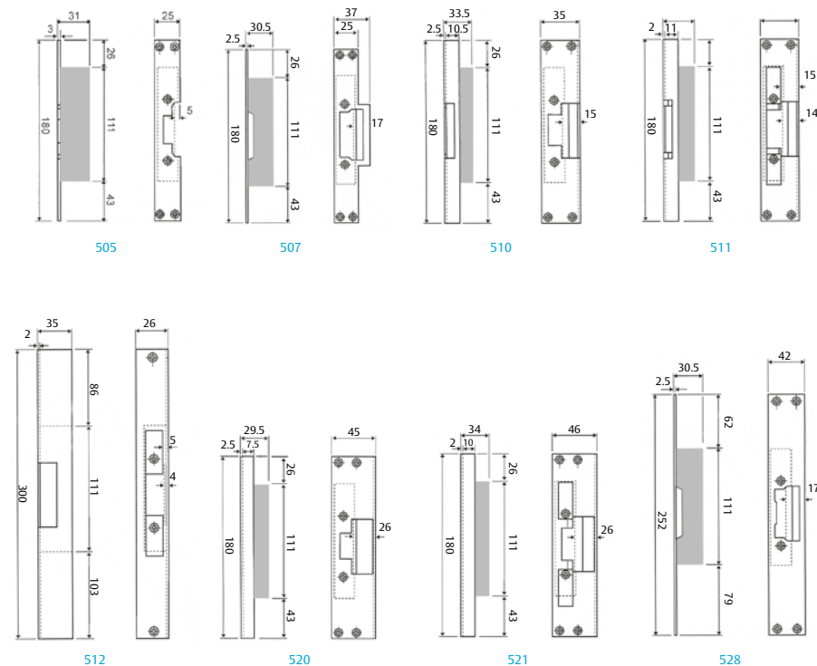
Dimensions in mm, not proportional
