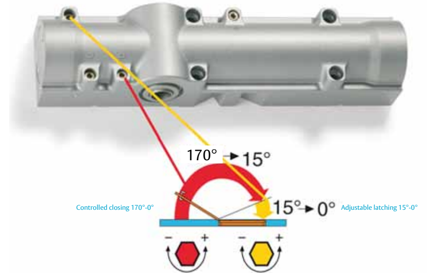
Adjusting latching and closing speed, delayed closing and back check.
