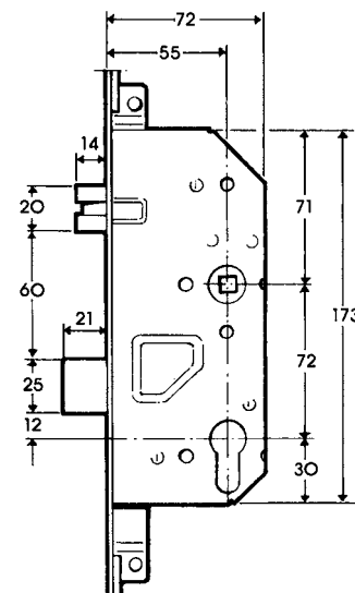
Lock case
