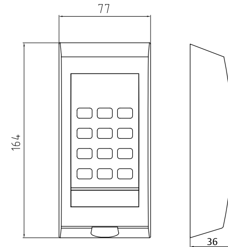
Dimension drawing
