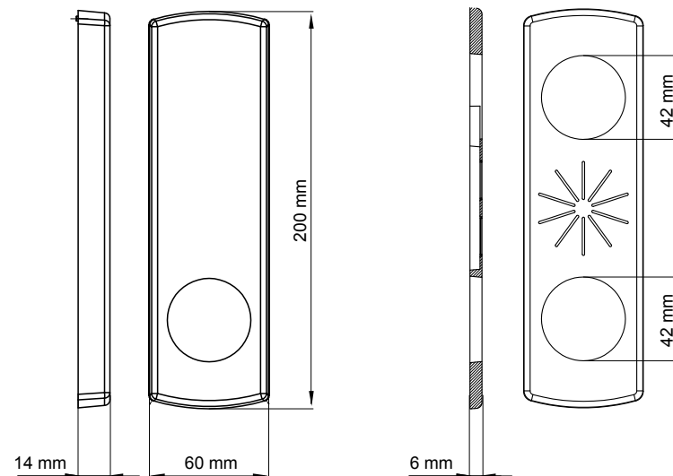
Dimension drawing
