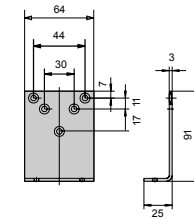
Parallel arm mounting plate A154
