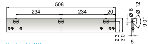
Mounting plate A115
