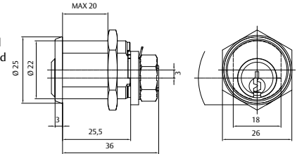
Measurement in mm
