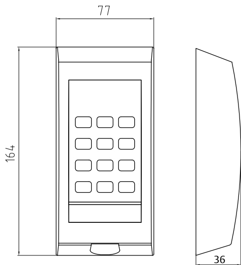
Dimension drawing
