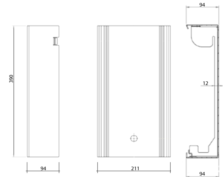
Dimension drawing
