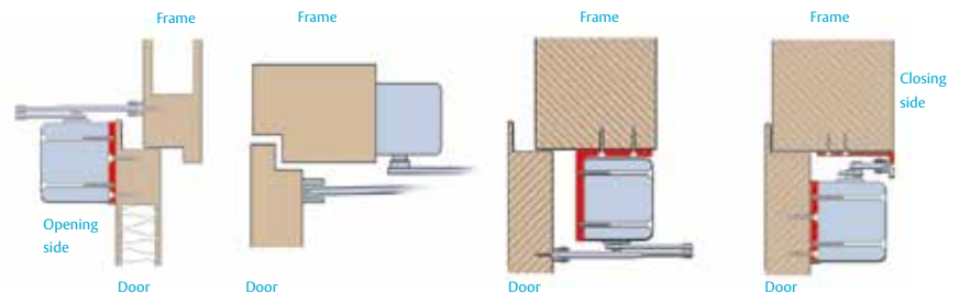
Normal mounting plate
