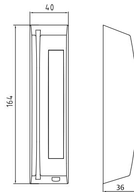
Dimension drawing
