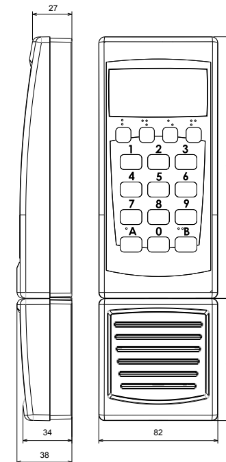
Dimension drawing
