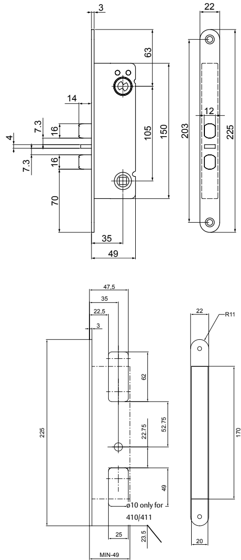
Dimensions in mm, not proportional
