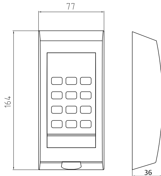
Dimension drawing
