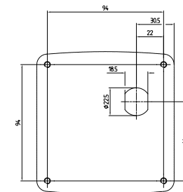
Hole preparation in mm
