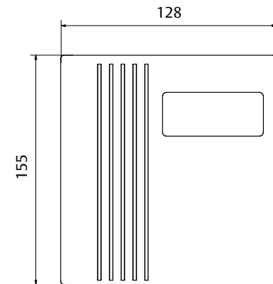
Dimension drawing LCU9101
