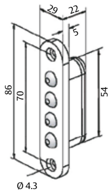
Dimensions in mm, not proportional
