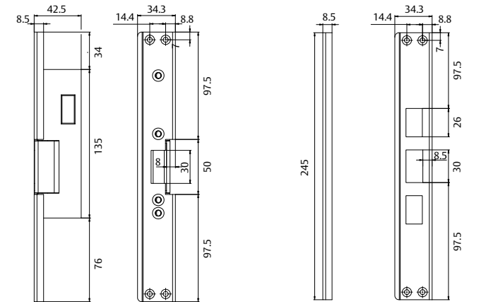
Faceplate 845 Strike plate 545
