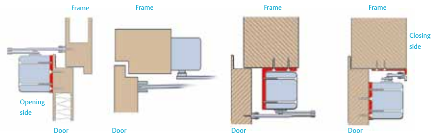
Normal mounting plate
