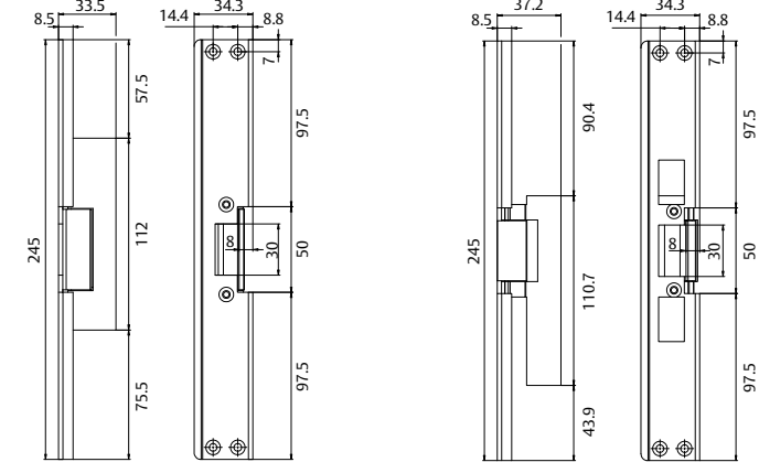
Faceplate 545
