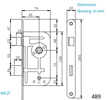
Dimension drawing in mm
