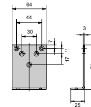
Parallel arm mounting plate A154
