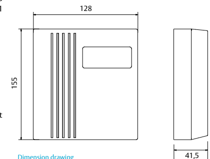
Dimension drawing
