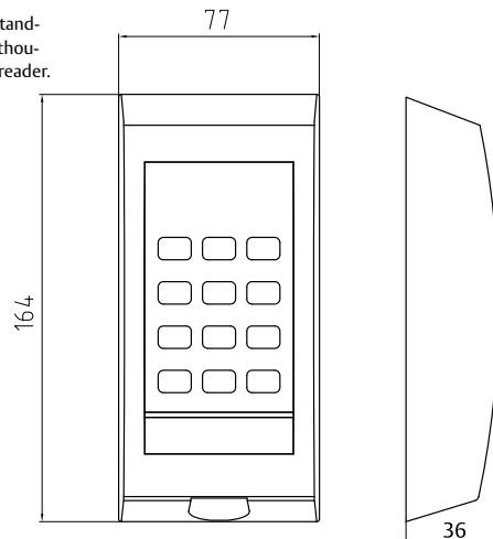
Dimension drawing
