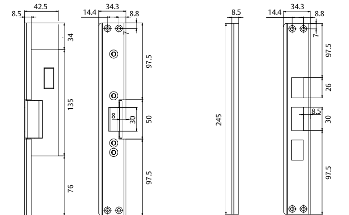
Faceplate 845
