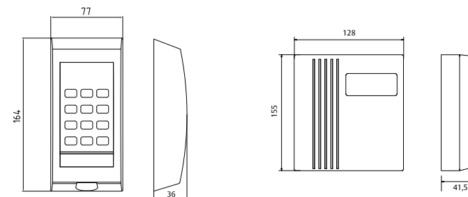
Dimension drawing
