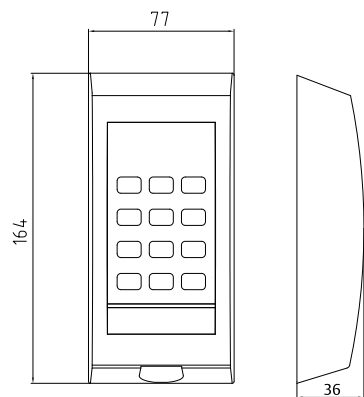
Dimension drawing
