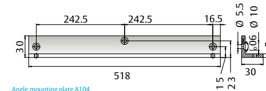
Angle mounting plate A104
