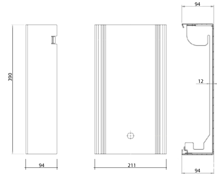
Dimension drawing LCU9016II
