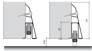
External mounting strip made of aluminium
